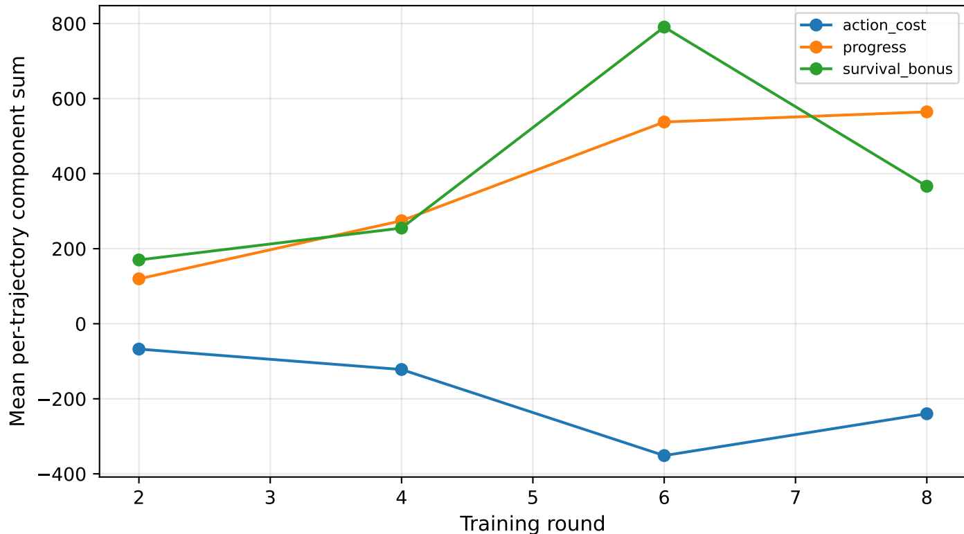
Walker2d-v4: reward components across rounds
