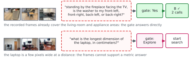
Figure 10: The exploration gate: covered questions are answered directly (top); insufficient coverage starts the search (bottom).
