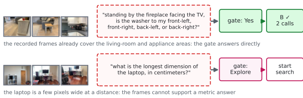
Figure 6: The exploration gate on two real questions. Top: the frames cover the queried areas, so the direct answer is returned after two calls. Bottom: the object’s size cannot be judged from distant frames, so the gate starts the search.
