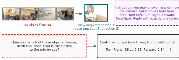
Figure 10: One camera-controller step. The valid moves are listed in the prompt, and the scores of all candidate actions are read from a single prefill pass, so a control step costs no answer decoding.
