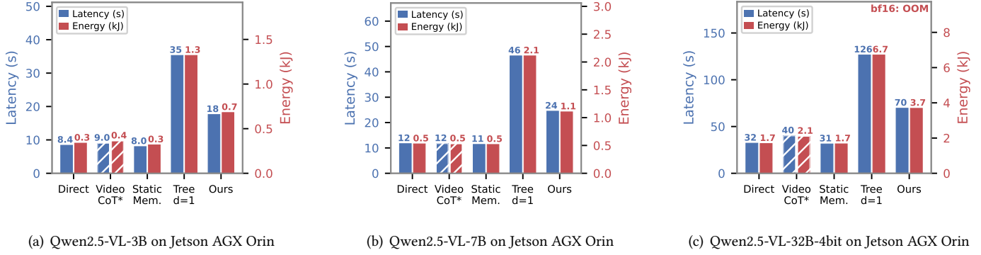
Figure 17: Measured per-question cost on Jetson AGX Orin with different VLM backbones (expected cost at the evaluation route mix). *Video-CoT is derived from the direct-input call plus the evaluation’s mean CoT decode length at the backbone’s measured decode rate; all other bars are full measured runs.
