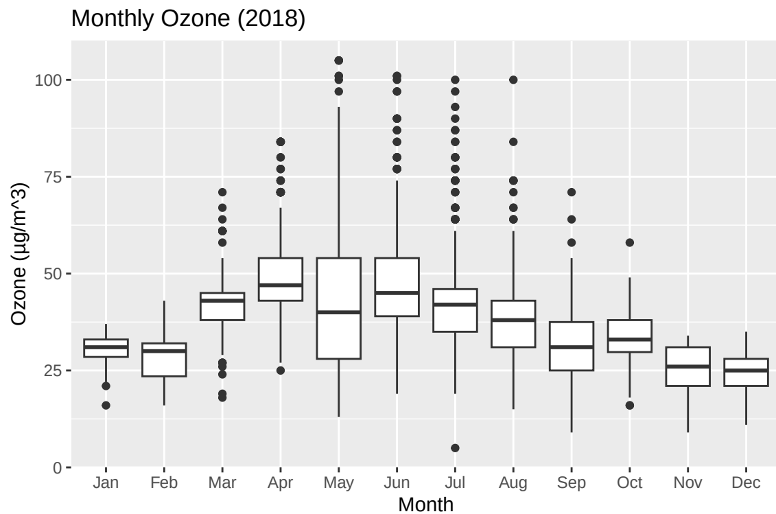
Figure 1: Monthly Ozone (2018)
