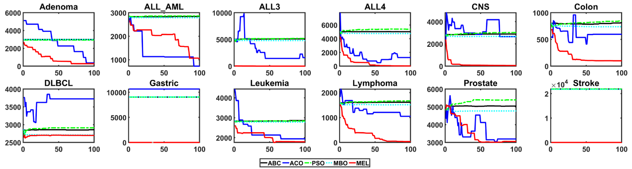
Fig. 3. Convergence Curves of Swarm-based EC Algorithms in Terms of the Size of Feature Subset.
