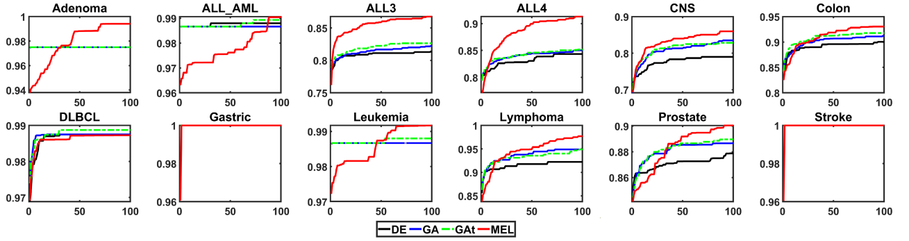
Fig. 6. Convergence Curves of Evolutionary Algorithms in Terms of Accuracy.
