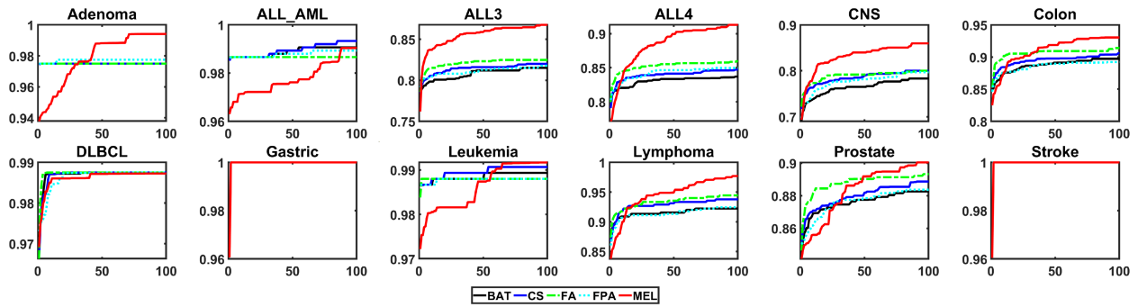
Fig. 4. Convergence Curves of Nature-inspired EC Algorithms in Terms of Accuracy.
