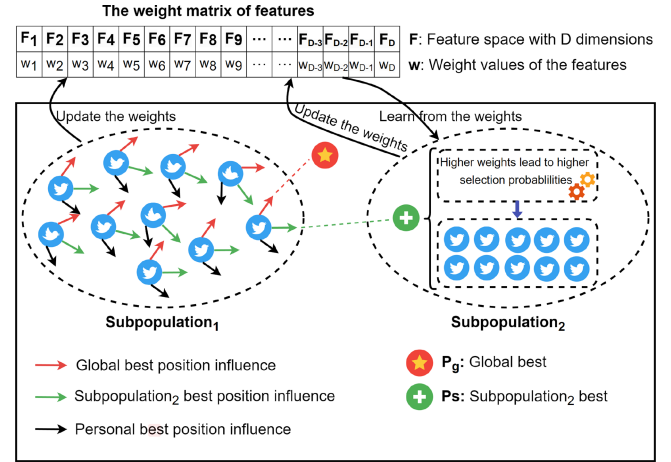
Fig. 1. Schematic diagram of the proposed MEL method. The parent population is divided into two subpopulations: Sub 1 learns the feature importance during evolution, and its search is affected by Sub 2 best. Sub 2 also learns the importance of features during evolution, and searches for the optimal feature subset based on the results learned from Sub 1 and Sub 2 . In particular, features with higher weights have a higher probability of being selected.
