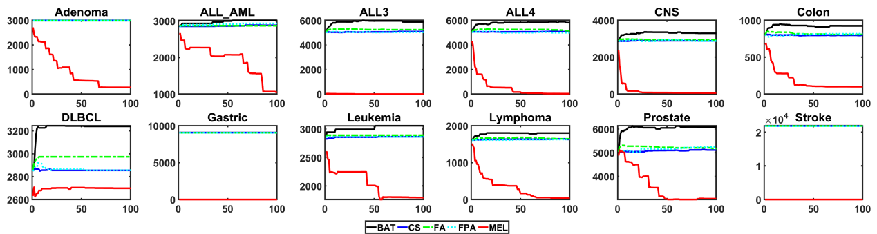
Fig. 5. Convergence Curves of Nature-inspired EC Algorithms in Terms of the Size of Feature Subset.
