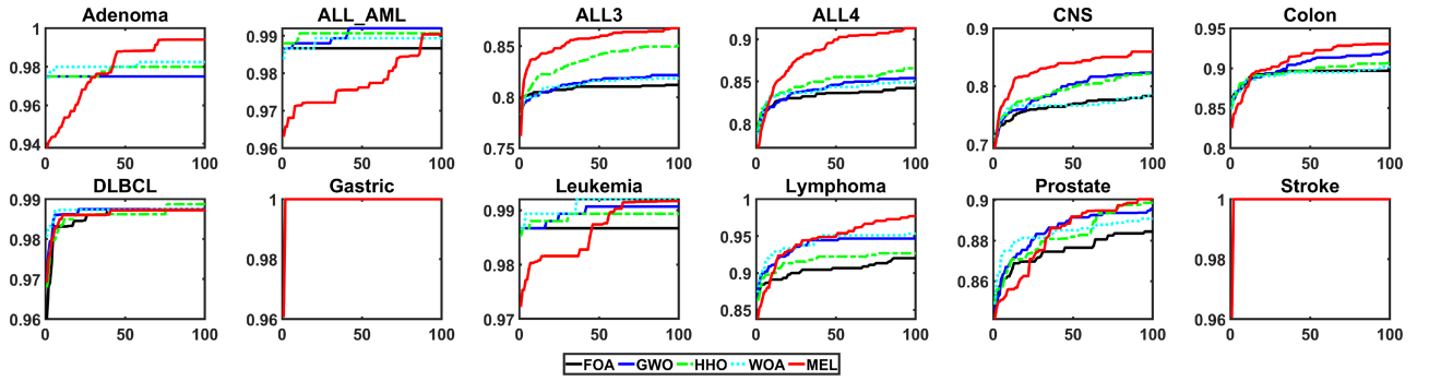
Fig. 8. Convergence Curves of Bio-stimulated EC Algorithms in Terms of Accuracy.
