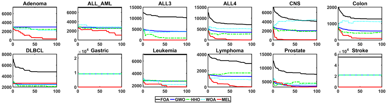
Fig. 9. Convergence Curves of Bio-stimulated EC Algorithms in Terms of the Size of Feature Subset.
