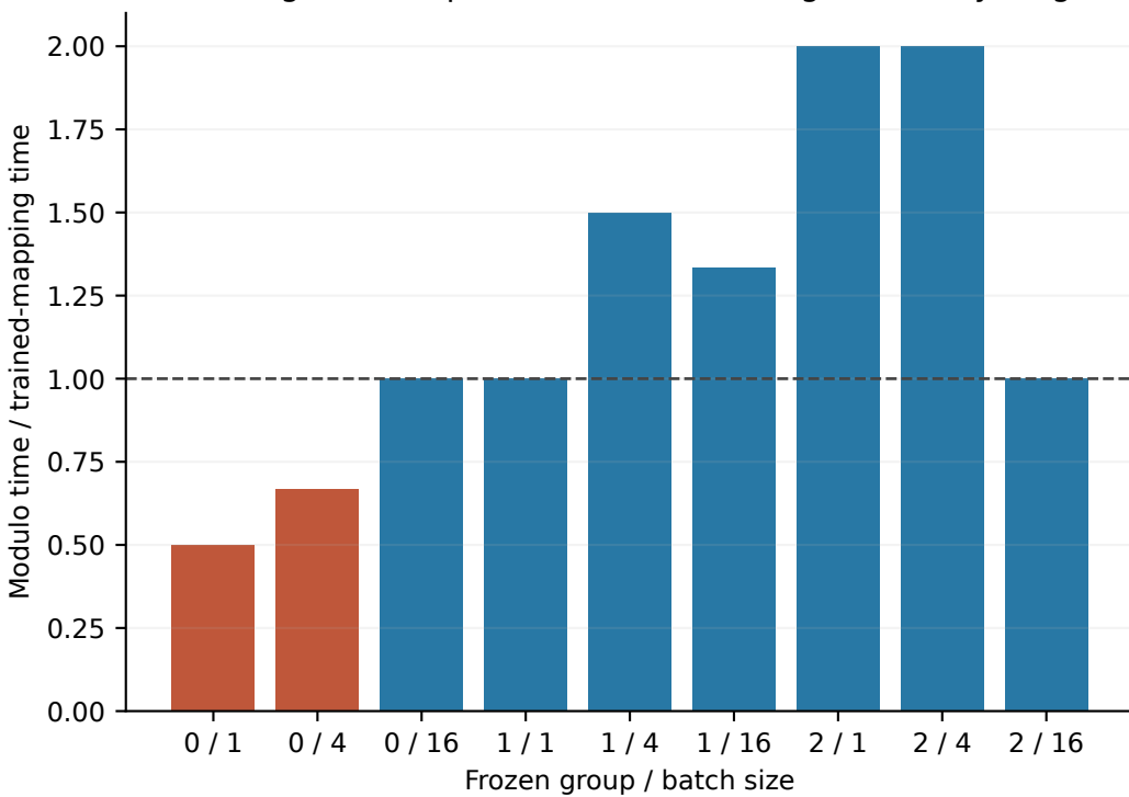
(c) Marginal-load placement is not enough for every stage
