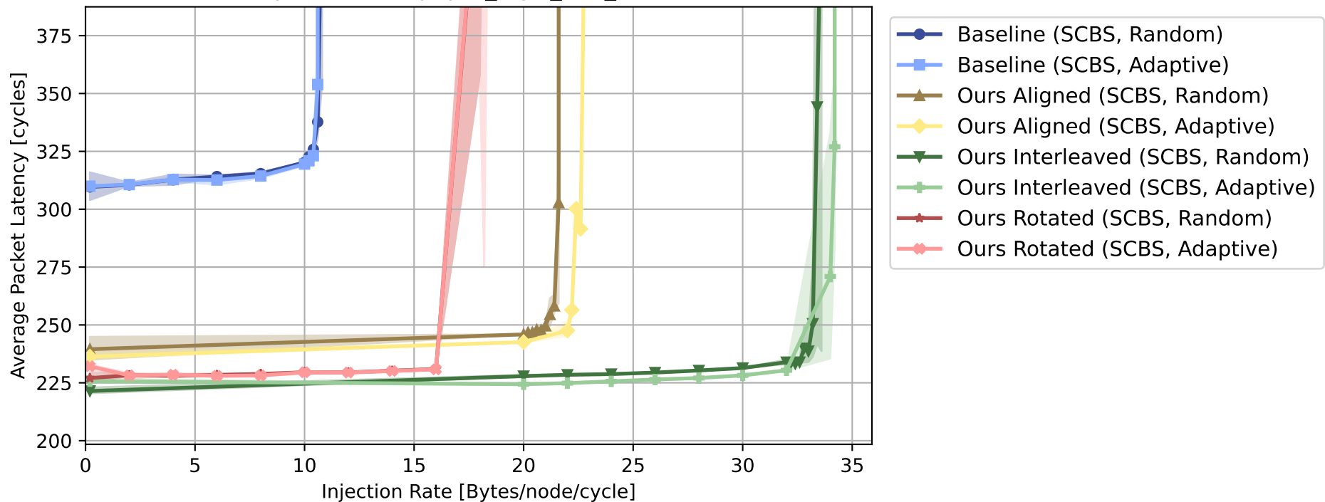
Latency vs Load of paper_logic_and_interconnect
