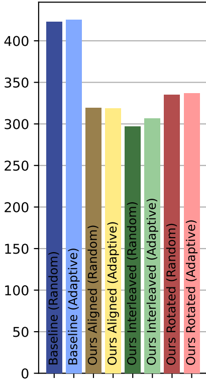
Energy per Byte at Saturation Throughput [pJ/Byte]
