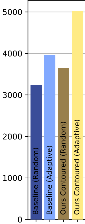
Network Power at Saturation Throughput [W]
