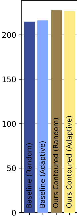
Energy per Byte at Saturation Throughput [p]/Byte]
