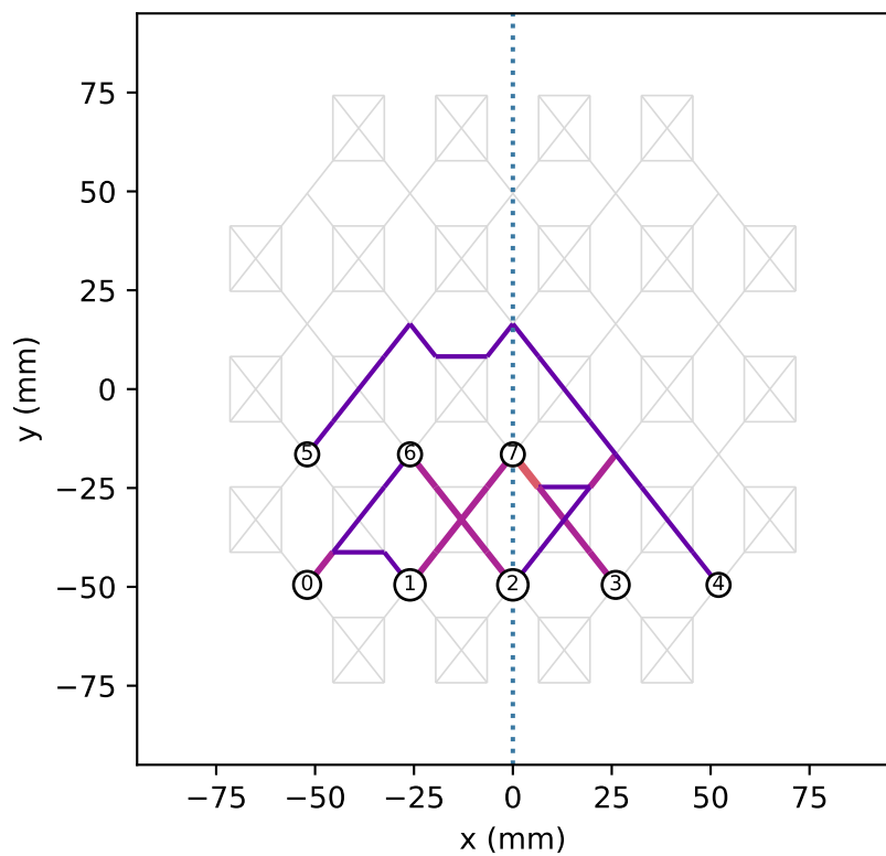
tree / Baseline
