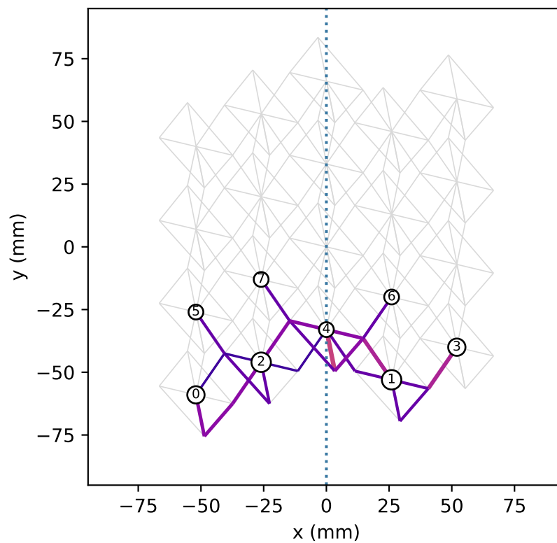
tree / Rotated
