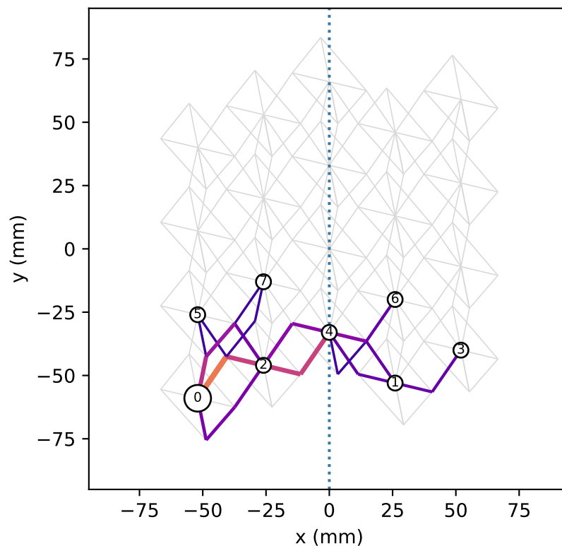
tree / Rotated
