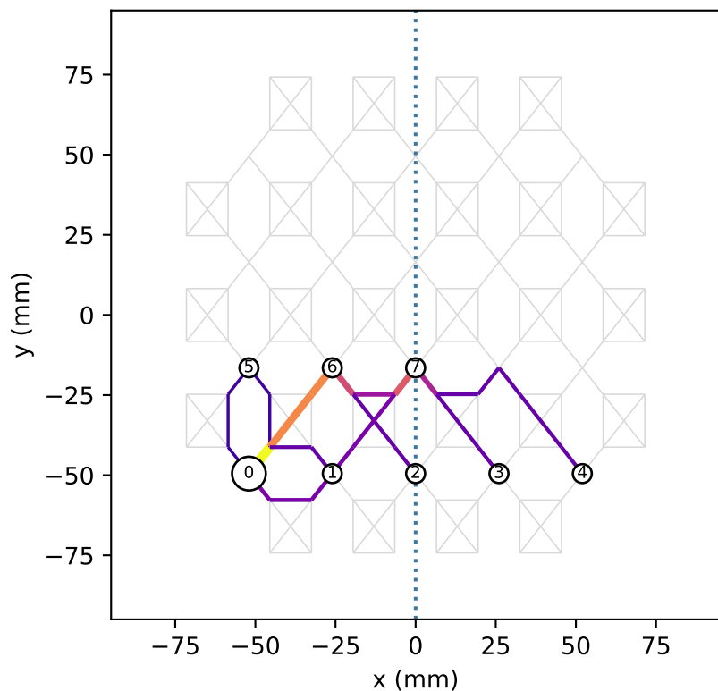
tree / Baseline
