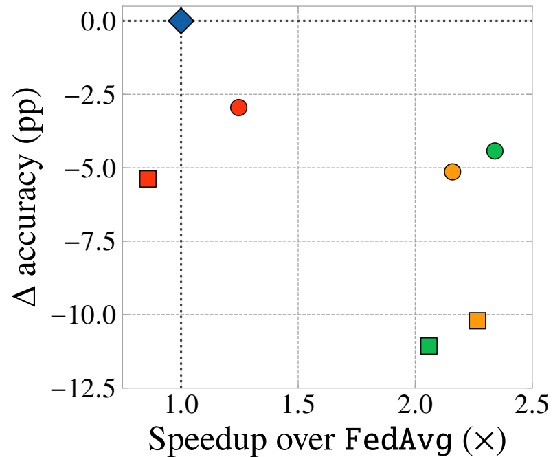
CIFAR-10
