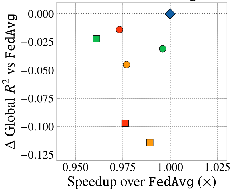
California Housing
