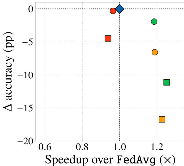
Fashion-MNIST
