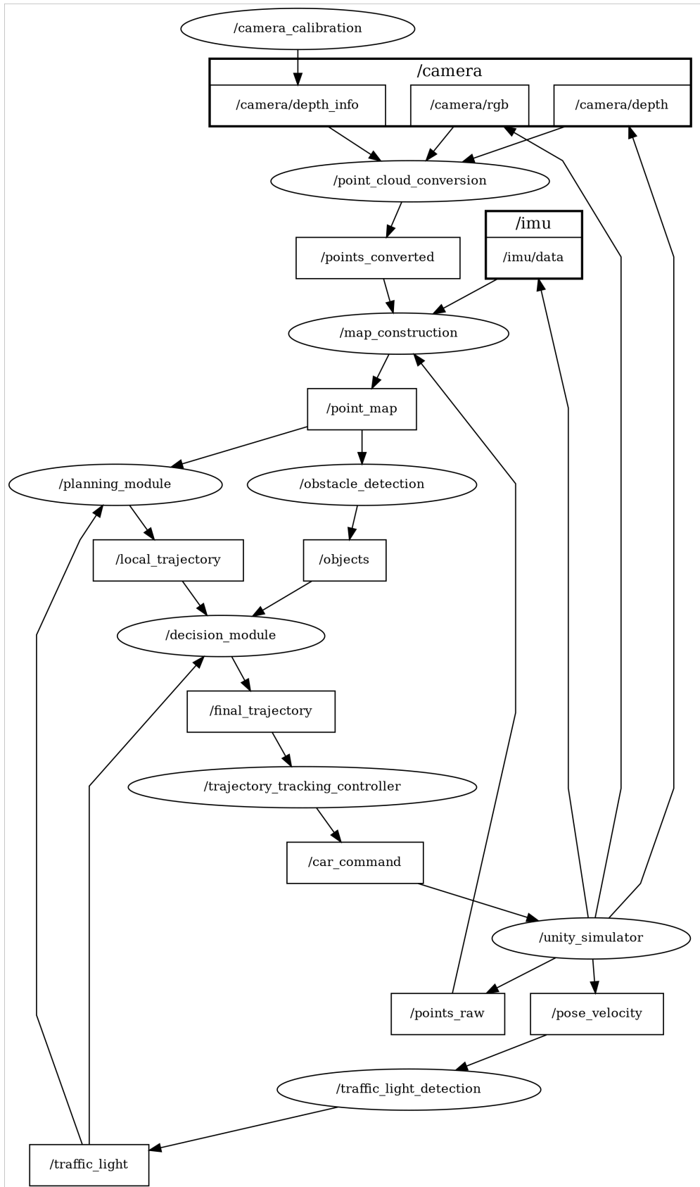
Figure 1: ROS Graph
