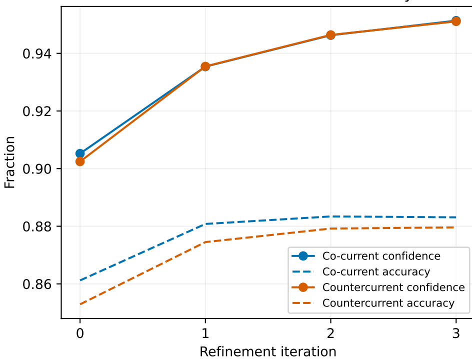
Full test set: confidence vs accuracy
