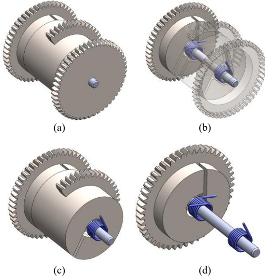
Fig. 3. The Idle-Stroke Gear.
