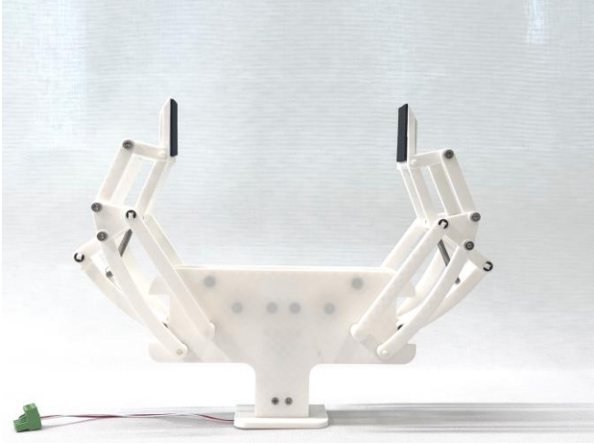
Fig. 1. Prototype of the proposed GLINT hand.
