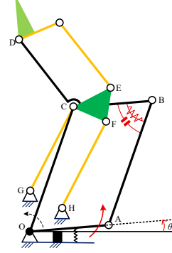
Fig. 4. Four-bar lifting unit with Idle-Stroke transmission.
