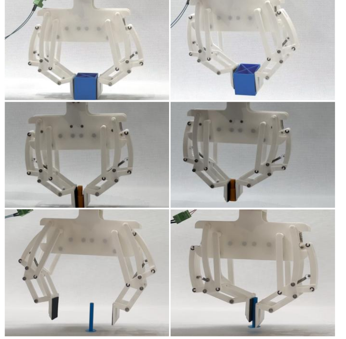
Fig. 6. Prototype and feasibility demonstration.
