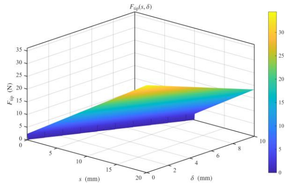
Fig. 5. Quasi-static force build-up across Idle and Engagement.
