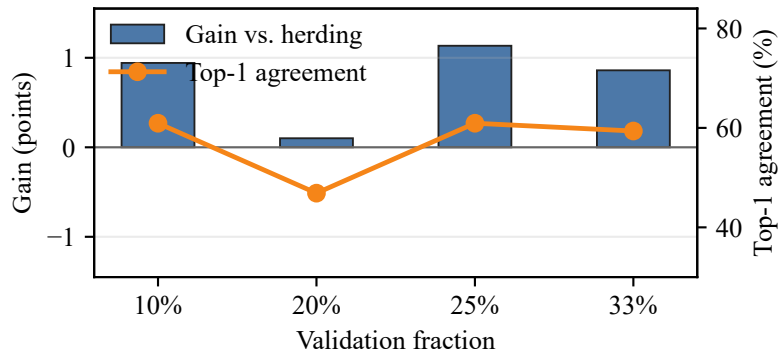
Validation-size reliability
