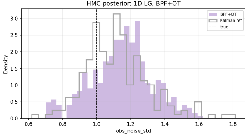
Figure 30: 1D LG HMC posterior: BPF+OT. Split- \hat{R} = 1.15 on this run (see Table 12), meaning the chain did not converge cleanly — the posterior shape should be read with that caveat.
