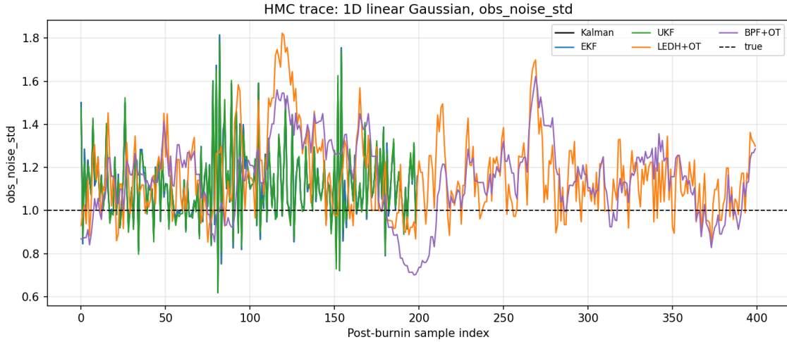
Figure 25: Post-burn-in chains for \sigma_{\text{obs}} on 1D LG. Kalman is the reference; the particle-filter chains should sit on the same posterior region.
