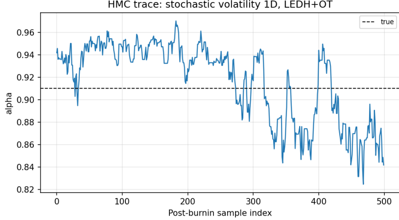
Figure 33: 1D stochastic volatility HMC post-burn-in trace for \alpha , LEDH+OT filter. Dashed reference line at the true value 0.91.
