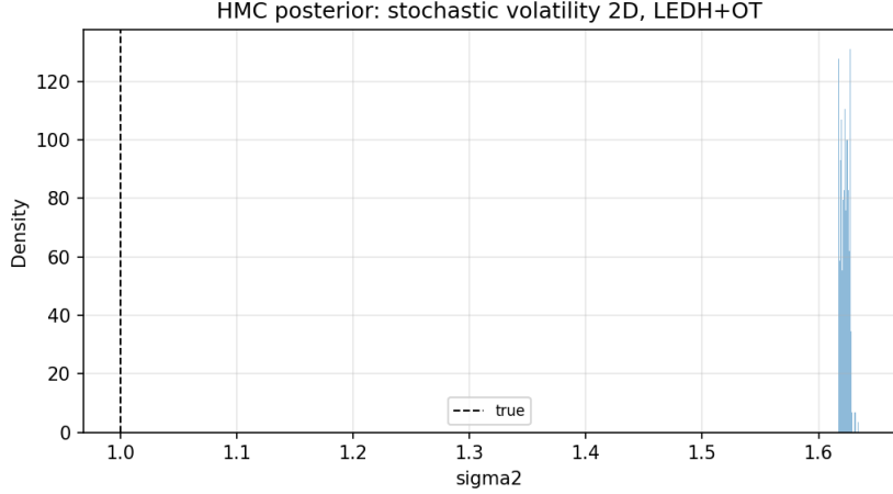
Figure 36: 2D stochastic volatility HMC marginal posterior for \sigma_2 , LEDH+OT filter. The posterior is broader than the SV1D and LG cases, reflecting the step-level gradient instability discussed below.
