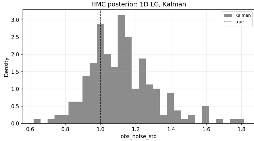
Figure 26: 1D LG HMC posterior: Kalman filter. This is the HMC reference other filters are compared against.
