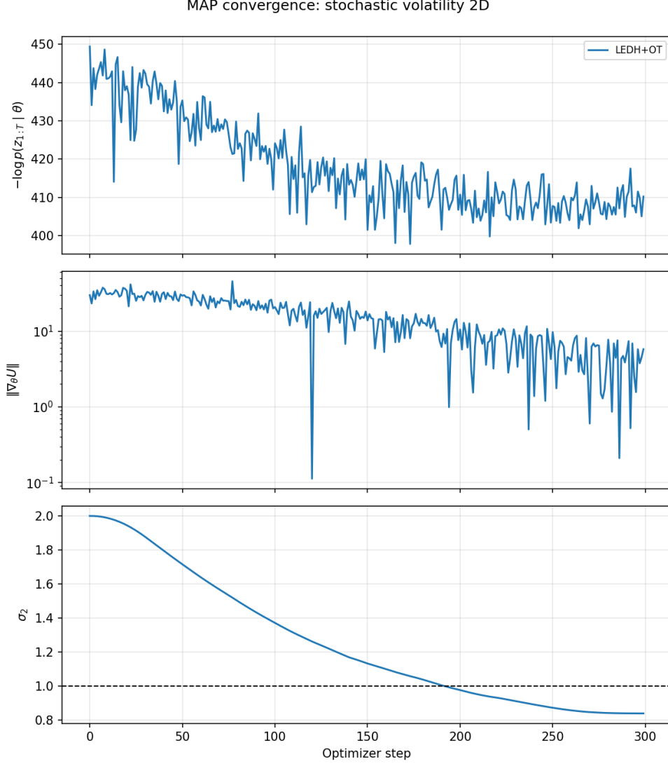
Figure 24: MAP convergence on 2D stochastic volatility with LEDH+OT, estimating \sigma_2 with true value 1.0. The MAP optimizer clears the filter-level objective; §6.5 shows why this is not enough for HMC.
