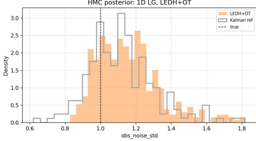
Figure 29: 1D LG HMC posterior: LEDH+OT. This is the main flow-filter HMC check.
