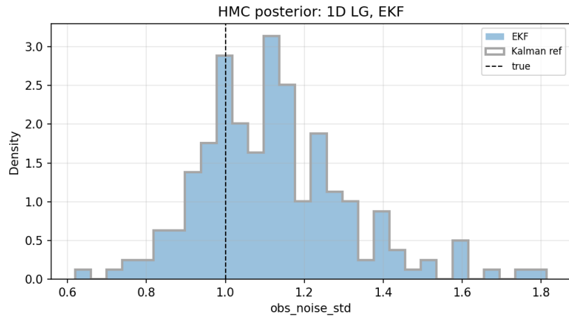
Figure 27: 1D LG HMC posterior: EKF. Kalman outline in grey, true value as dashed vertical.
