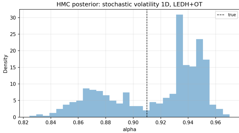
Figure 34: 1D stochastic volatility HMC marginal posterior for \alpha , LEDH+OT filter.
