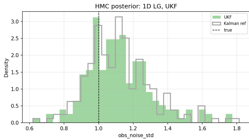
Figure 28: 1D LG HMC posterior: UKF.
