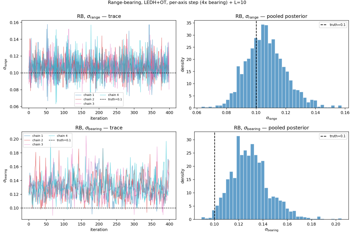
Figure 37: Range-bearing four-chain HMC, post-burn-in. Top row: \sigma_{\text{range}} . Bottom row: \sigma_{\text{bearing}} . Left column: four-chain traces. Right column: pooled marginal posteriors with dashed lines at the true values (0.10 for both).
