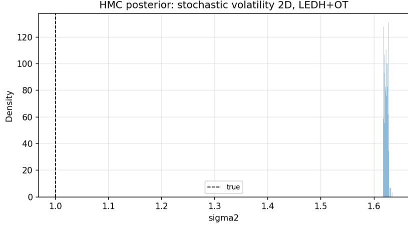
Figure 39: 2D stochastic volatility HMC marginal posterior for \sigma_2 , LEDH+OT filter. The posterior is broader than the SV1D and LG cases, reflecting the step-level gradient instability discussed below.
