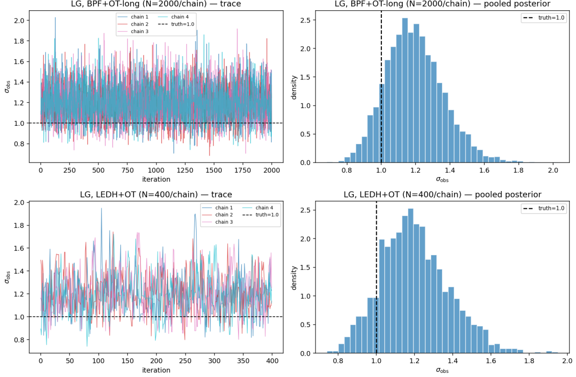
Figure 35: 1D LG four-chain HMC, post-burn-in. Top row: BPF+OT with extended sample budget (2000 per chain). Bottom row: LEDH+OT (400 per chain). Left column: traces, four chains overlaid in distinct colors. Right column: pooled marginal posterior with truth at 1.0 as the dashed vertical line.
