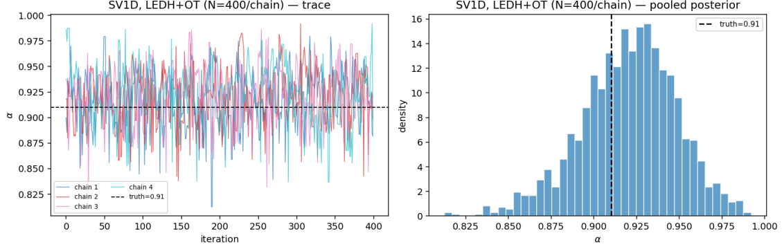
Figure 36: 1D SV four-chain HMC, post-burn-in. Left: traces, four chains in distinct colors. Right: pooled marginal posterior for \alpha , dashed line at truth 0.91.
