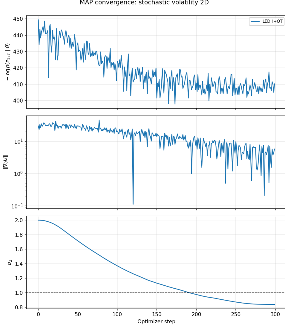
Figure 24: MAP convergence on 2D stochastic volatility with LEDH+OT, estimating \sigma_2 with true value 1.0. The MAP optimizer clears the filter-level objective; §6.6 shows why this is not enough for HMC.
