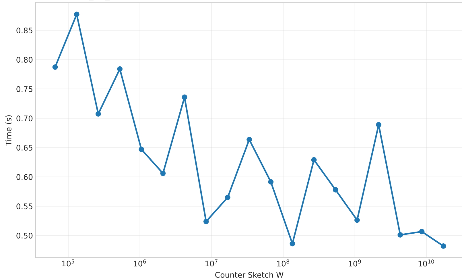
adult_ml_v2 - Time vs Counter Sketch W (speedup: 5.05x-29.66x, mean=9.56x)
