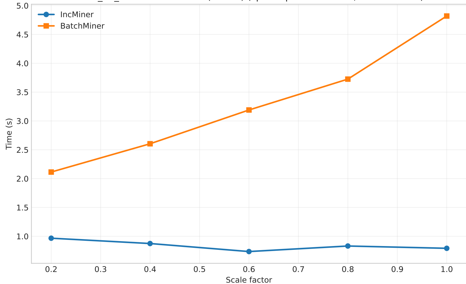
adult_ml_v2 - Time vs Scale (SCALE) (speedup: 2.19x-6.09x, mean=4.01x)
