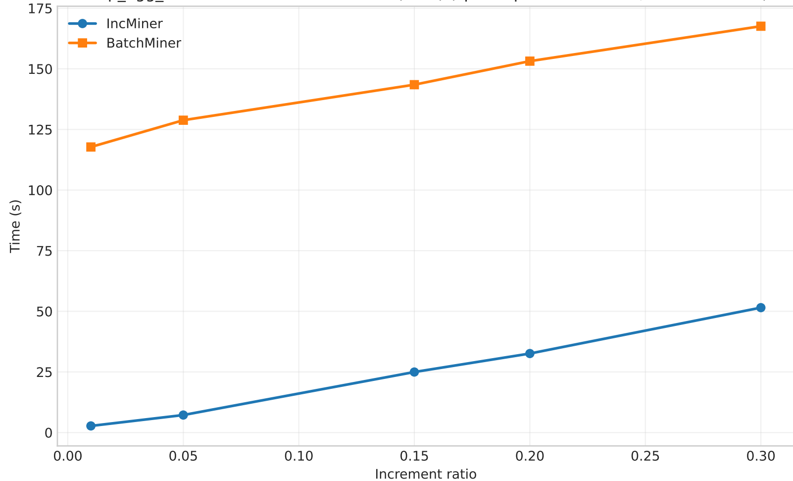
dblp_agg_v2 - Time vs Increment Ratio (ADD) (speedup: 3.25x-43.02x, mean=14.91x)
