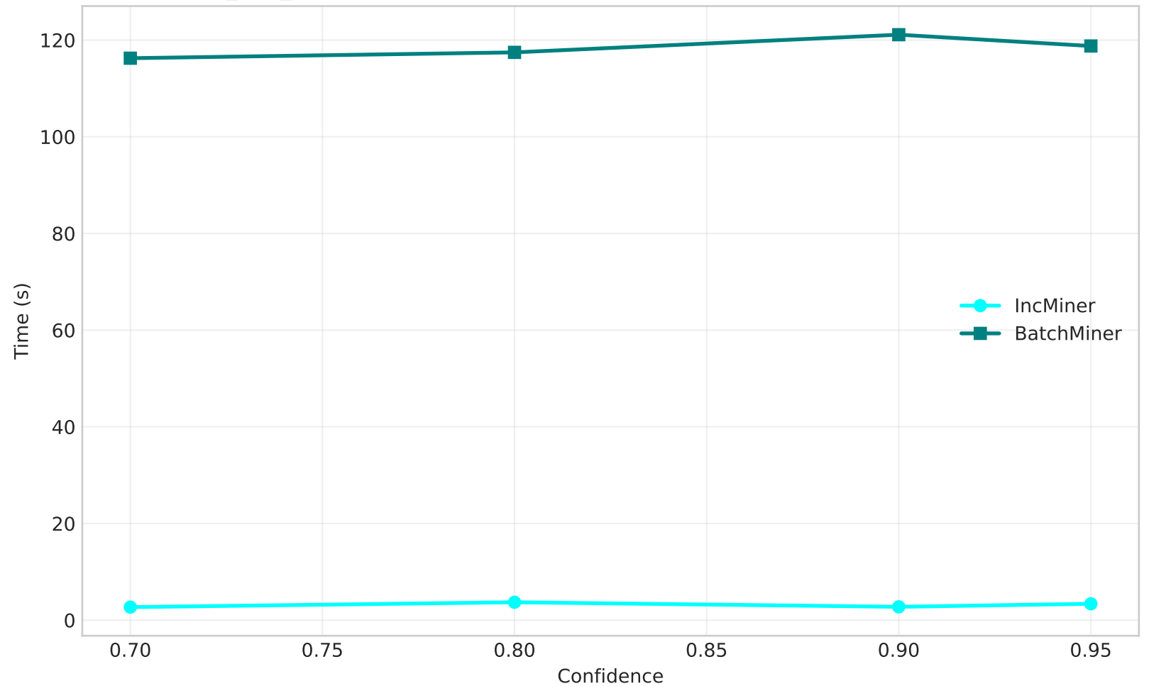
dblp_agg_v2 - Time vs Confidence (speedup: 31.67x-43.81x, mean=38.38x)
