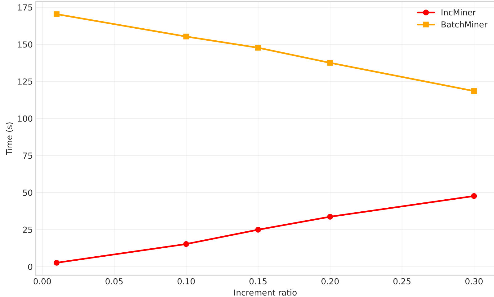
dblp_agg_v2 - Time vs Increment Ratio (DELETE) (speedup: 2.49x-64.45x, mean=17.42x)
