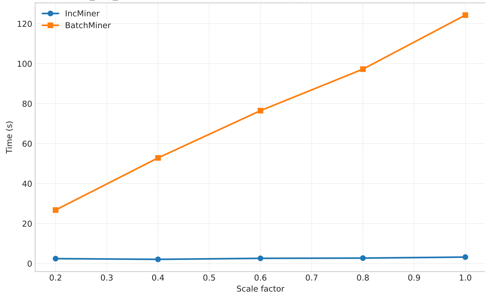
dblp_agg_v2 - Time vs Scale (SCALE) (speedup: 10.94x-38.66x, mean=28.07x)
