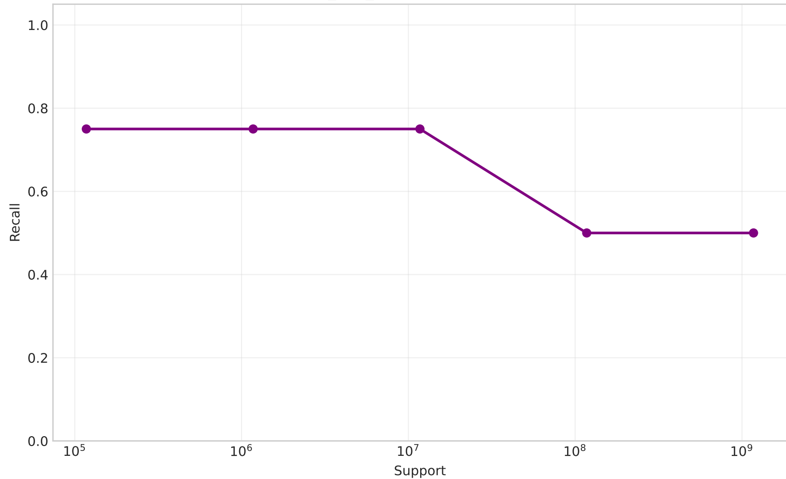
dblp_agg_v2 - Recall vs Support
