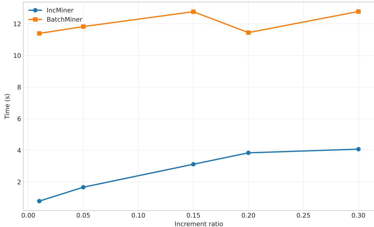
hospital_ml_v2 - Time vs Increment Ratio (ADD) (speedup: 2.98x-14.42x, mean=6.34x)
