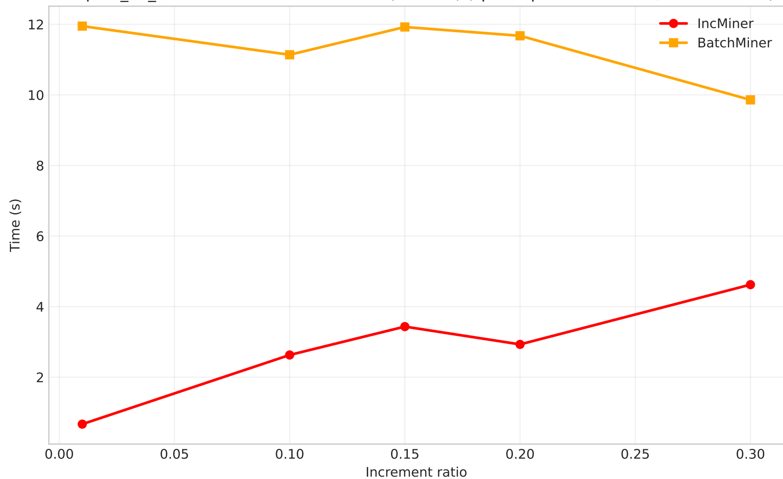
hospital_ml_v2 - Time vs Increment Ratio (DELETE) (speedup: 2.13x-17.85x, mean=6.34x)
