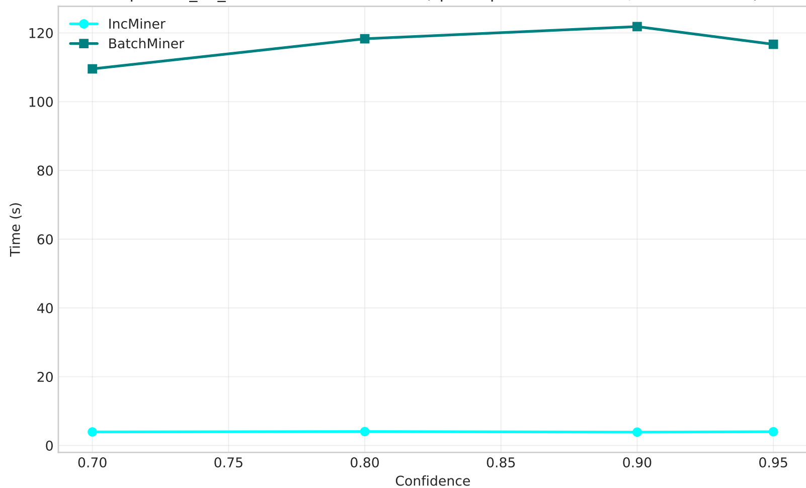
inspection_ml_v2 - Time vs Confidence (speedup: 27.86x-31.41x, mean=29.45x)
