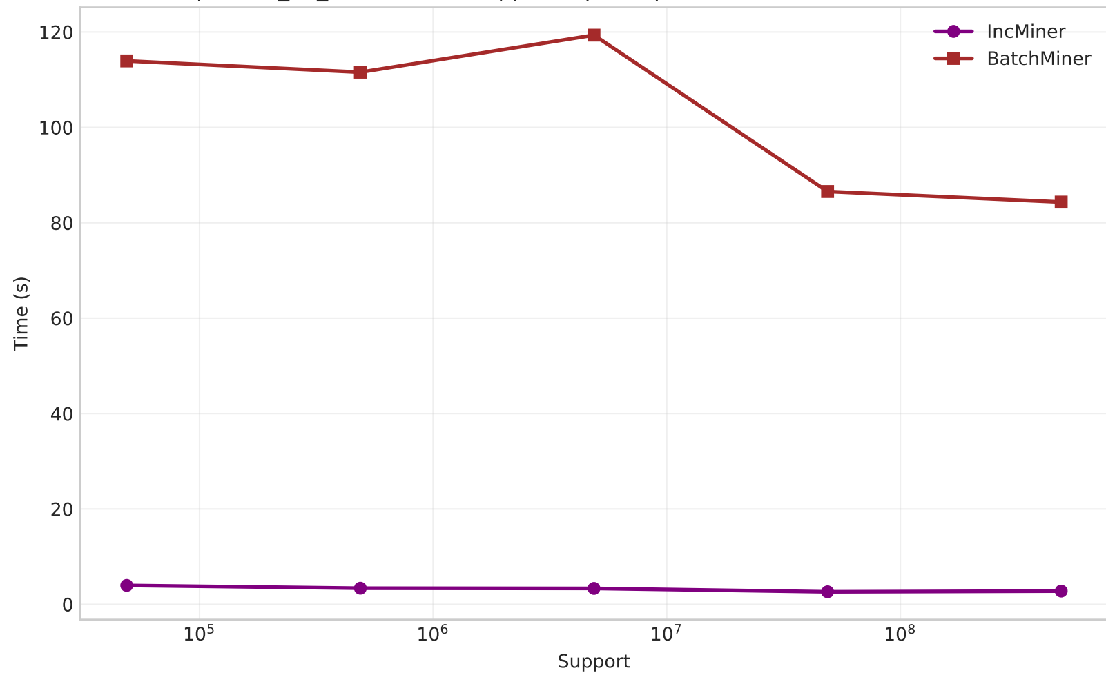
inspection_ml_v2 - Time vs Support (speedup: 28.74x-35.77x, mean=32.17x)
