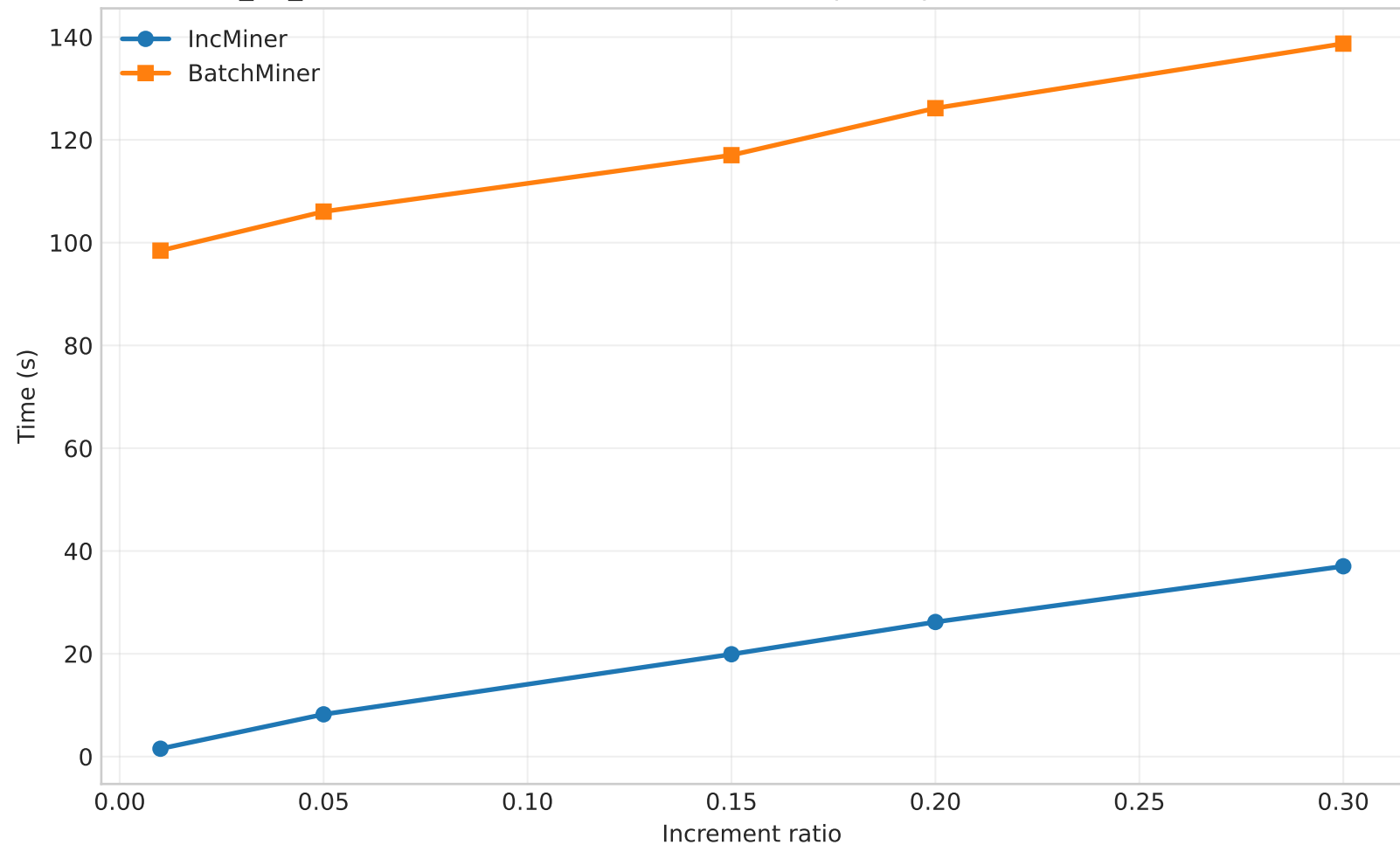
ncvoter_ml_v2 - Time vs Increment Ratio (ADD) (speedup: 3.75x-64.36x, mean=18.34x)
