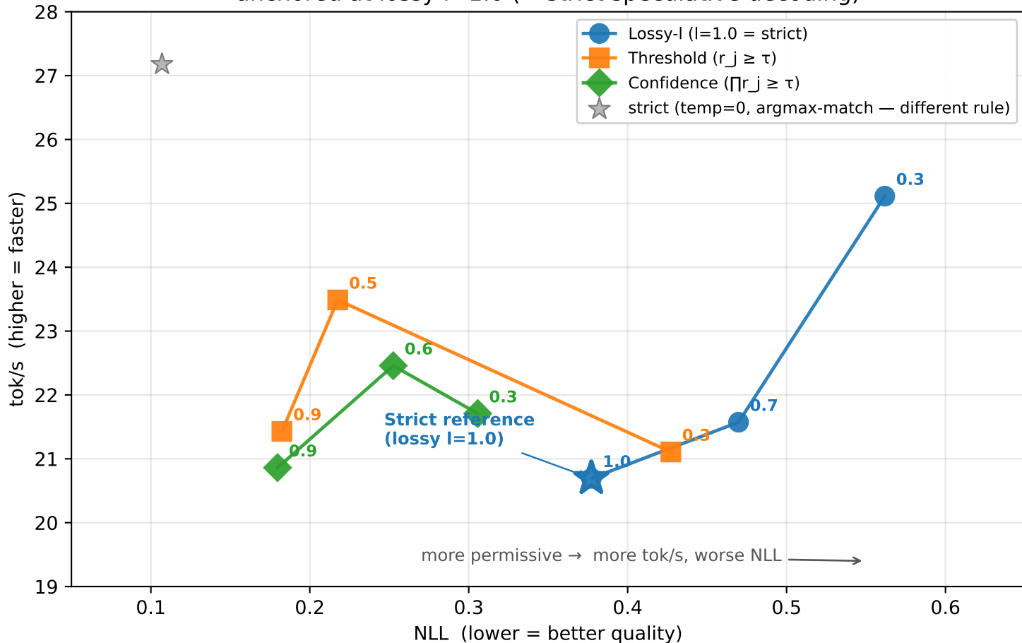
Throughput-Quality Trade-off on OpenWebText anchored at lossy l=1.0 (= strict speculative decoding)
