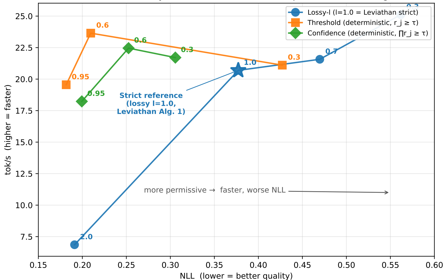
Throughput-Quality Trade-off on OpenWebText anchored at lossy l=1.0 (= Leviathan strict speculative decoding)
