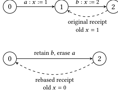
Fig. 1. Receipt rebasing after selective erasure. Solid arrows are forward executions; dashed arrows use occurrence receipts. The upper receipt belongs to the original predecessor and is stale in the lower replay.
