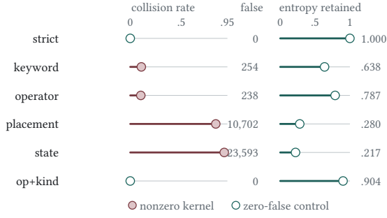
Figure 5: Projection information profile. Rose bars mark nonzero projection kernels; false-pair counts give witness denominators, while teal controls keep zero false pairs.
