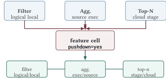
Figure 1: Projection loss in optimizer comparison. Distinct public contracts collapse to the same feature cell; treating that cell as equality creates a false comparison, while OptSem-C preserves the fields that separate it.
