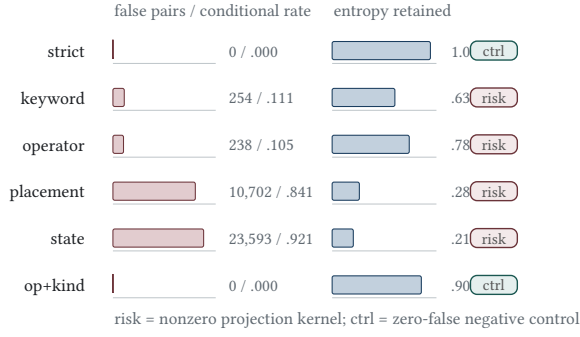
Figure 5: Projection information profile. Coarse projections induce contract collisions and lose signature entropy; controls retain zero pairwise collisions.
