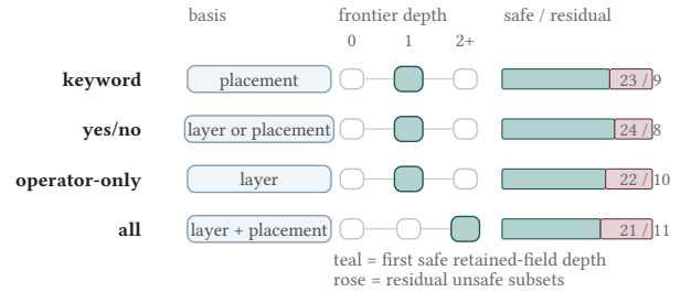
Figure 6: Semantic frontier over the core field lattice. Single projections cross the frontier at one field; the joint scope first becomes safe at layer+placement.
