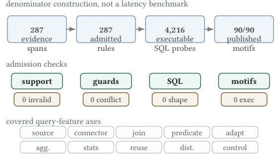
Figure 3: Corpus, benchmark, and execution denominators. The same grounded denominator carries source evidence, generated probes, admission checks, and published-motif coverage.
