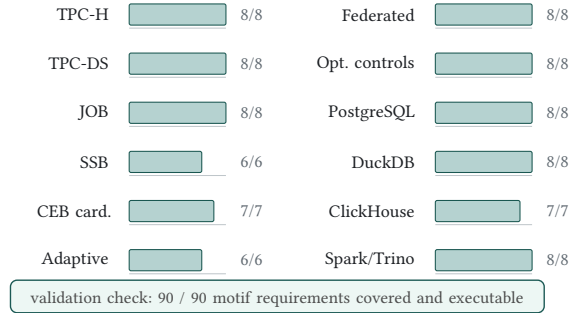
Figure 4: Published optimizer-motif denominator. The generated probe space covers 90 motifs across 12 recognizable optimizer and benchmark families, with every motif mapped to executable validation probes.
