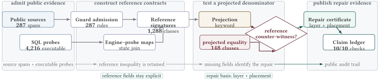
Figure 2: OptSem-C’s contract-comparison dataflow. Public sources and executable probes are admitted into reference signatures before a projected vocabulary is trusted; the rose gate exposes projected equality that contradicts reference inequality. The 148 keyword classes include 81 multi-reference classes and 254 false pairs (Table 7); each collision is tied to evidence, a counter-witness, and retained fields.
