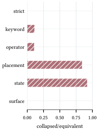
projection kernel
