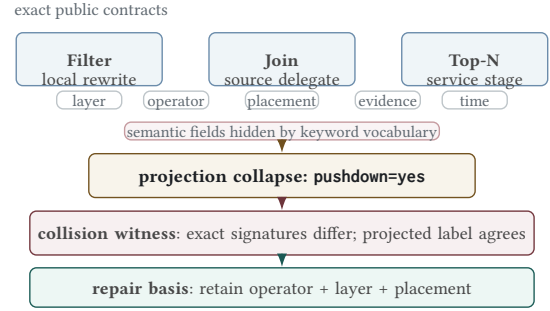
Figure 1: Projection loss in optimizer comparison. A feature-name matrix turns non-equivalent public optimizer contracts into the same apparent capability; OptSem-C records the hidden semantic fields that split the false comparison cell.
