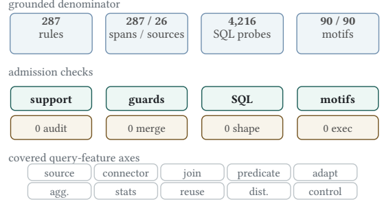
Figure 3: Corpus, benchmark, and execution denominators. Every mainline rule is public-evidence grounded, every generated SQL probe executes in the validation catalog, and every external optimizer motif has executable probe support.
