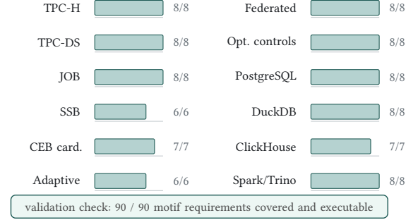
Figure 4: External optimizer-motif denominator. The generated probe space covers 90 motifs across 12 recognizable optimizer and benchmark families, with every motif mapped to executable validation probes.
