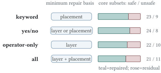
Figure 6: Semantic frontier over the core field lattice. Single fields repair the headline one-projection scopes, but the joint scope requires a layer+placement basis; safe and unsafe core subsets are counted by exhaustive finite enumeration.
