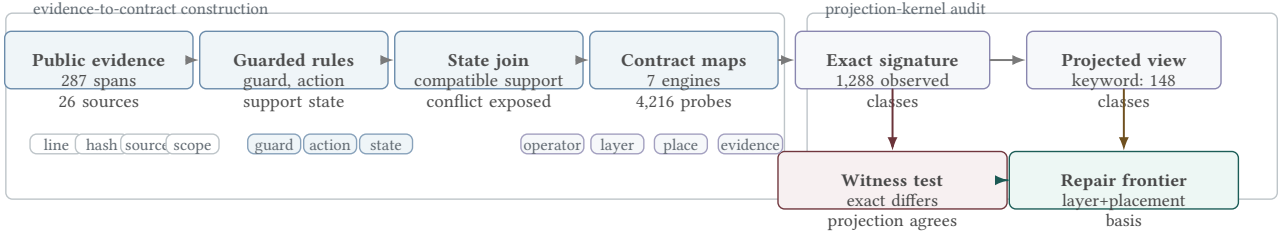
Figure 2: Contract-comparison pipeline. Public evidence becomes guarded modal rules and exact per-engine/per-probe signatures; a projected comparison is audited by a finite witness test, and nontrivial kernels produce minimum semantic repair frontiers.
