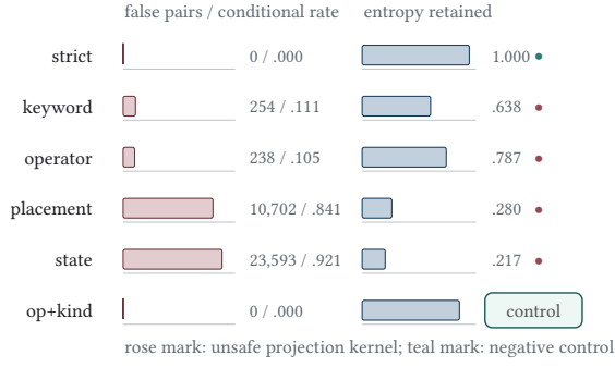
Figure 5: Projection information profile. Coarse projections induce contract collisions and lose signature entropy; strict comparison and the operator-kind surface are negative controls with zero pairwise collisions, while single-field vocabularies create large kernels.
