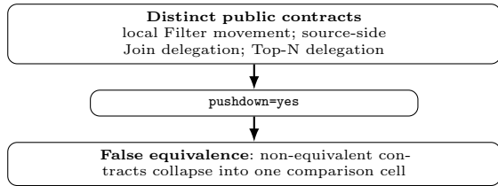
Figure 1: Projection loss in optimizer comparison. A feature-name matrix turns non-equivalent public optimizer contracts into the same apparent capability. OptSem-C preserves the semantic fields that distinguish them.
