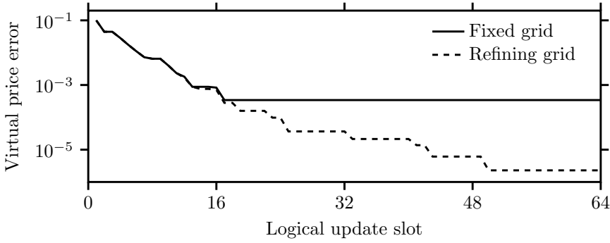
FIG. 2. Exact two-link experiment with D = 2 , initial price (4/5, 1) , alternating updates, and fixed or refining quantization. The curve is virtual-price error, not packet-network performance.
