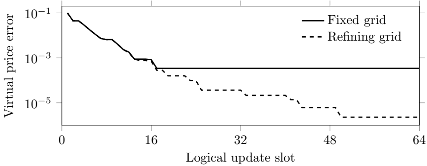
FIG. 2. Exact two-link experiment with D = 2 , initial price (4/5, 1) , alternating updates, and fixed or refining quantization. The curve is virtual-price error, not packet-network performance.
