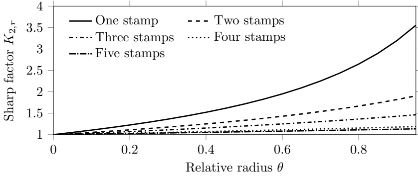
FIG. 1. Sharp support-two factors from one through five stamps. The fifth curve is K_{2,5} = 8/(8 - \theta) .
