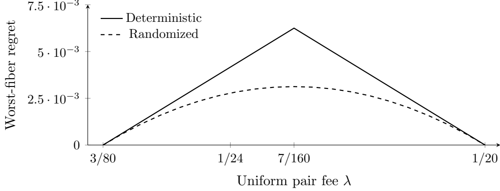
Figure 2: Exact deterministic and randomized deficiencies on the fixed three-item fiber as the uniform pair fee varies. Both are positive in the open interval (3/80, 1/20) and vanish at its endpoints. Randomization reduces, but does not eliminate, the information loss. Data are rational evaluations of Theorem 22; lines connect display samples.
