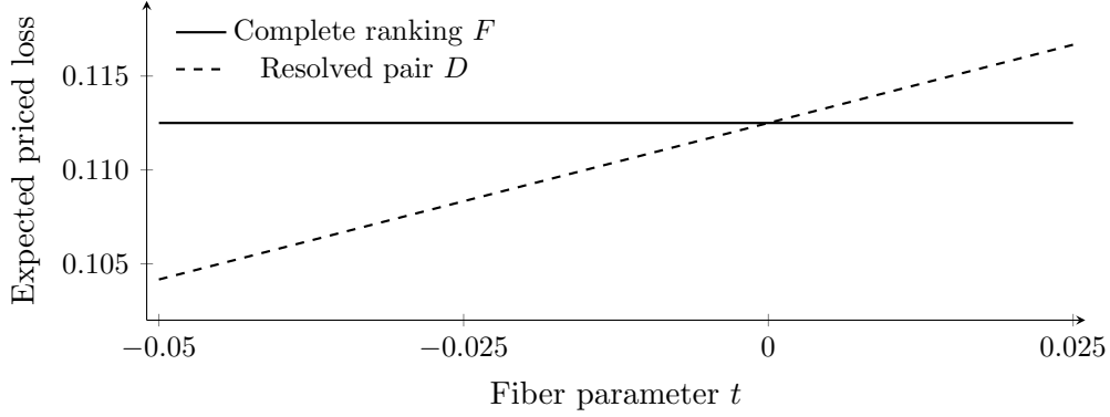
Figure 1: Risks on the entire quadratic-moment fiber at \lambda = 1/24 . The horizontal curve is the best complete-ranking risk; the increasing curve is the risk of 1 \mid \{2, 3\} . Their lower envelope is the Bayes risk. The common quadratic report cannot distinguish any horizontal location. Decimal tick labels are display conversions of the exact rational endpoints.
