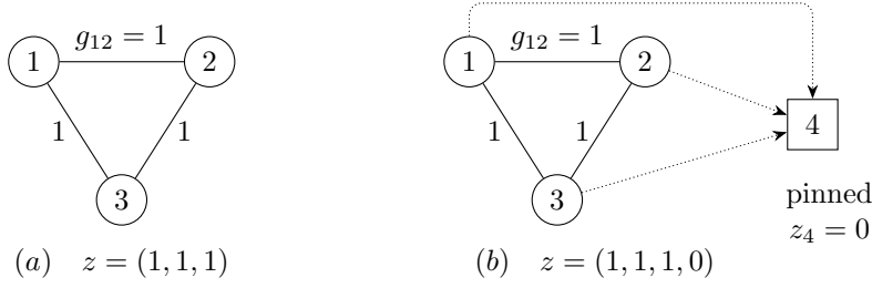
Figure 1: Two ambiguity structures. On the left, a balanced three-coordinate component has one direction supported on all three vertices, so its distance is three. On the right, an anchor is pinned by one-sided pair entries while the original three-coordinate component stays free. This is the distance-three construction in dimension four. Solid edges carry nonzero reciprocal gains; dotted arrows represent pinning information, not equality constraints. The graph describes diagonal changes, not causal relationships.
