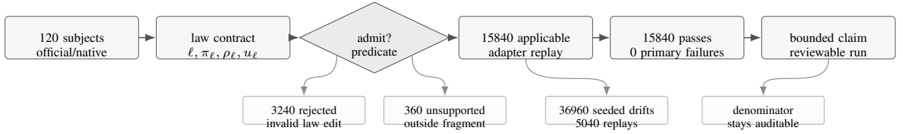
Fig. 2. Evidence flow. A law contract becomes a counted regression row only after the predicate gate admits the before/after slice; rejected edits, unsupported fragments, and seeded controls remain visible but outside the primary pass denominator.
