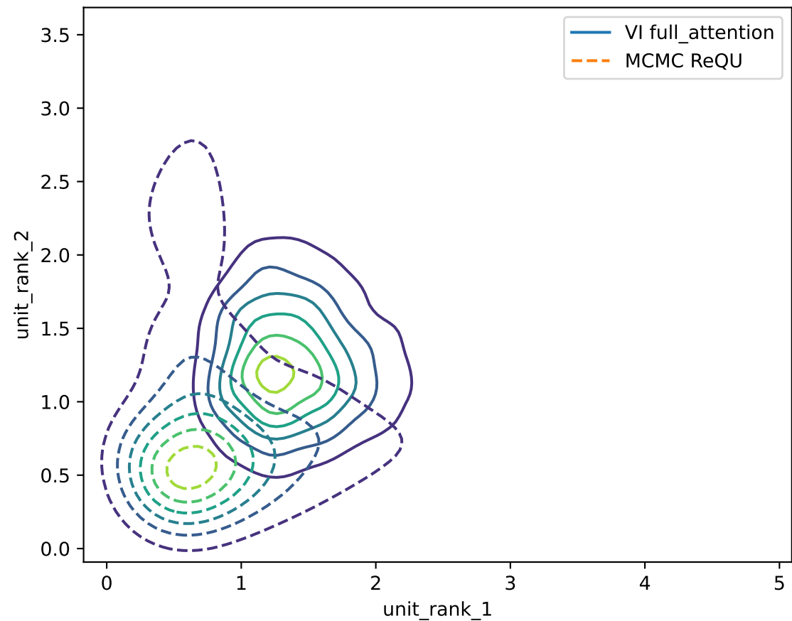
full attention vs matched MCMC
