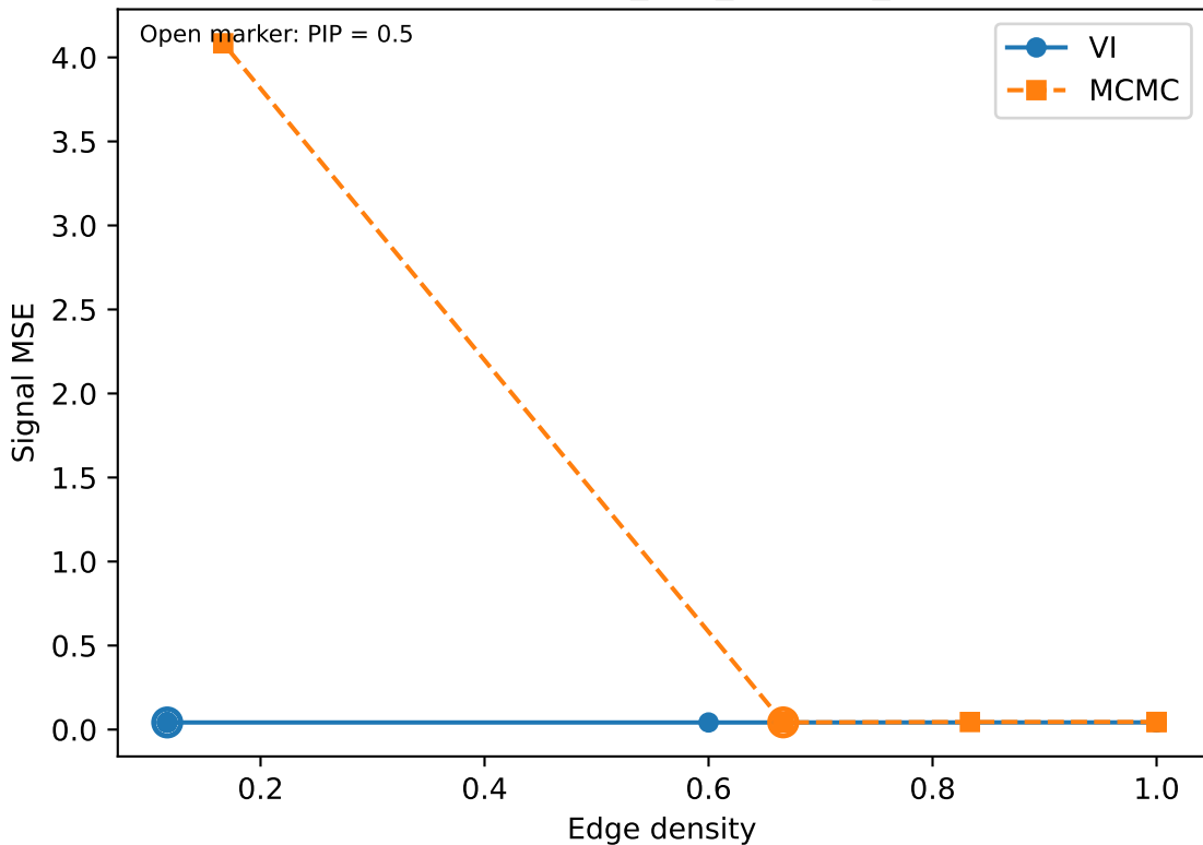
stacked: feature_unit_induced_edge
