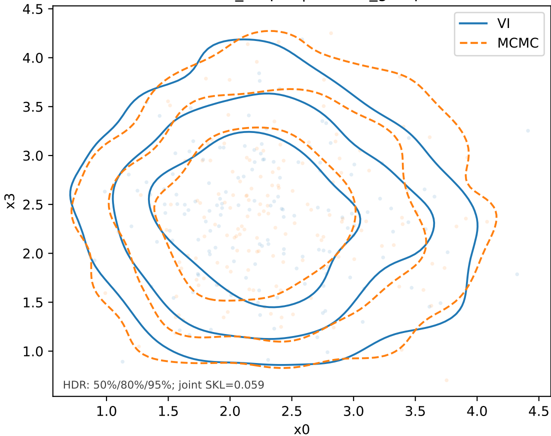
embed_output | feature_group
