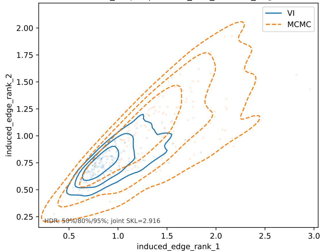
embed_output | feature_unit_induced_edge
